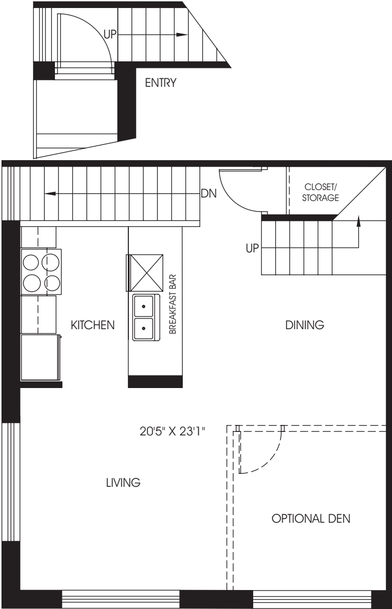
MAIN FLOOR
