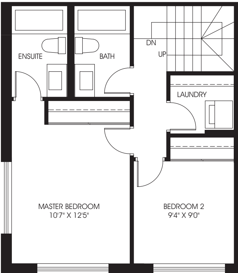
UPPER FLOOR
